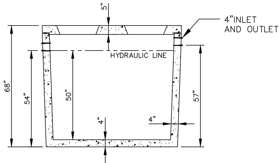
SECTION VIEW
