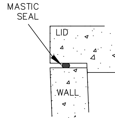
SEAL DETAIL
