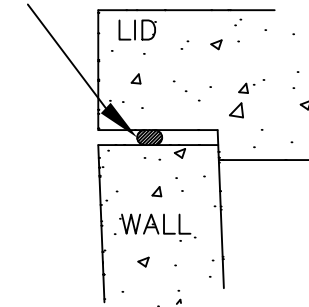
SEAL DETAIL
