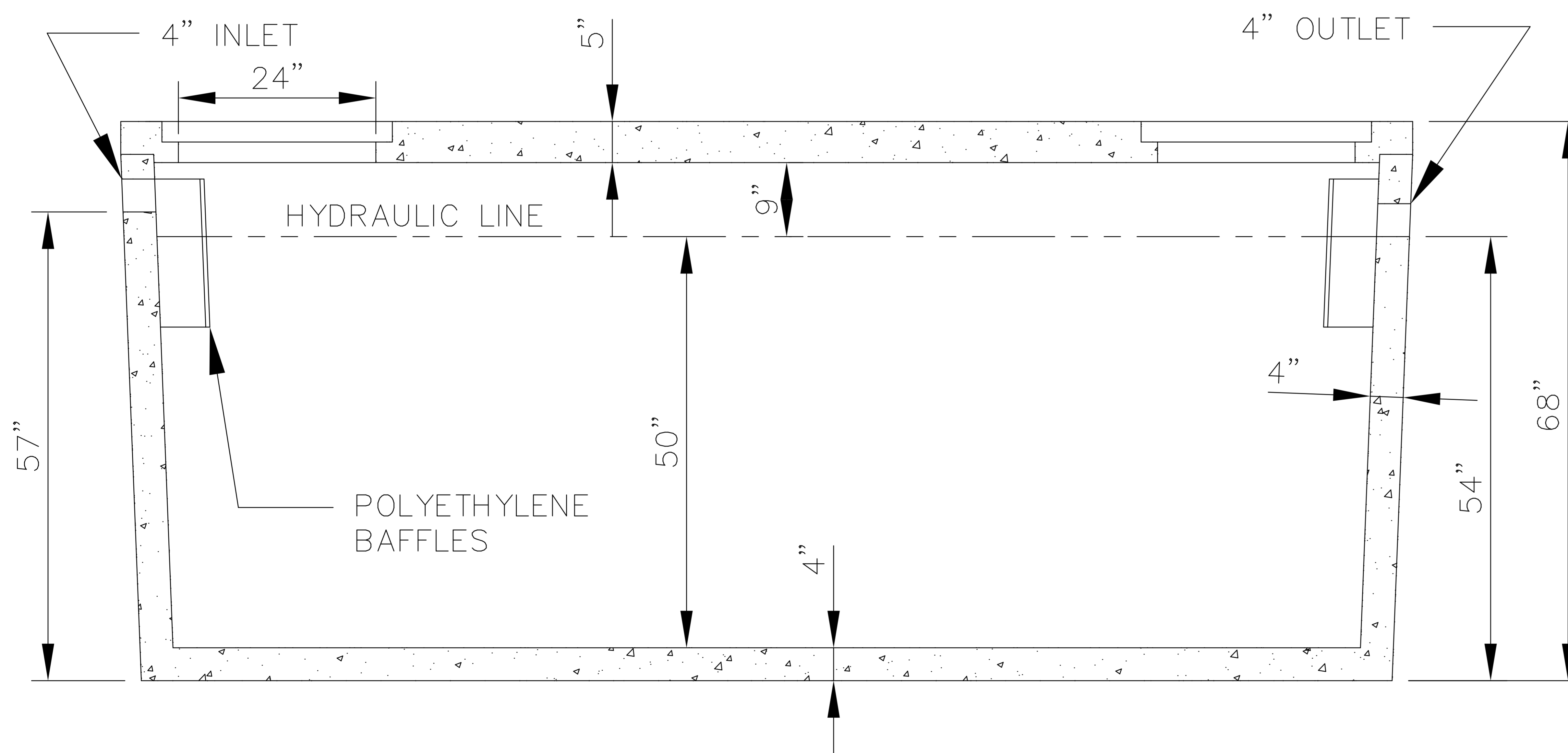
SECTION VIEW
