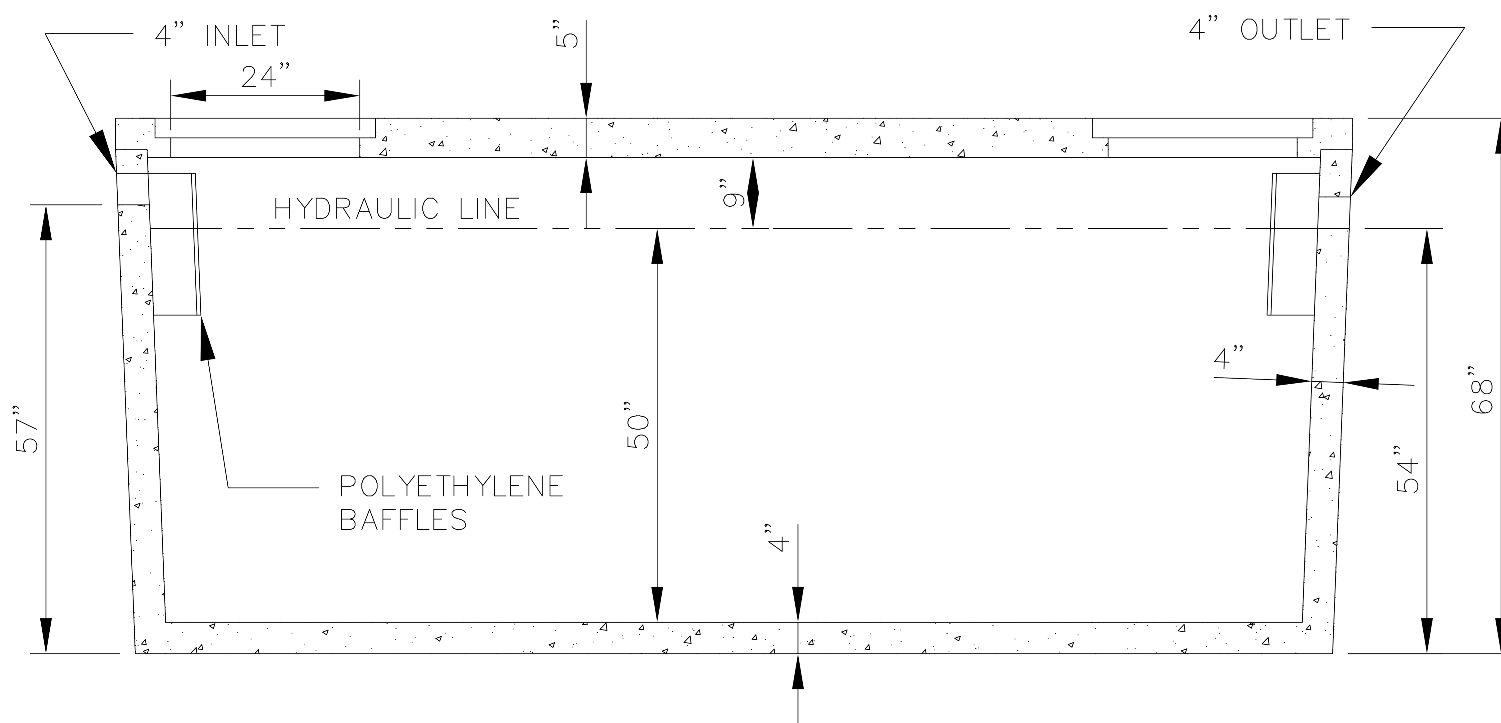
SECTION VIEW
