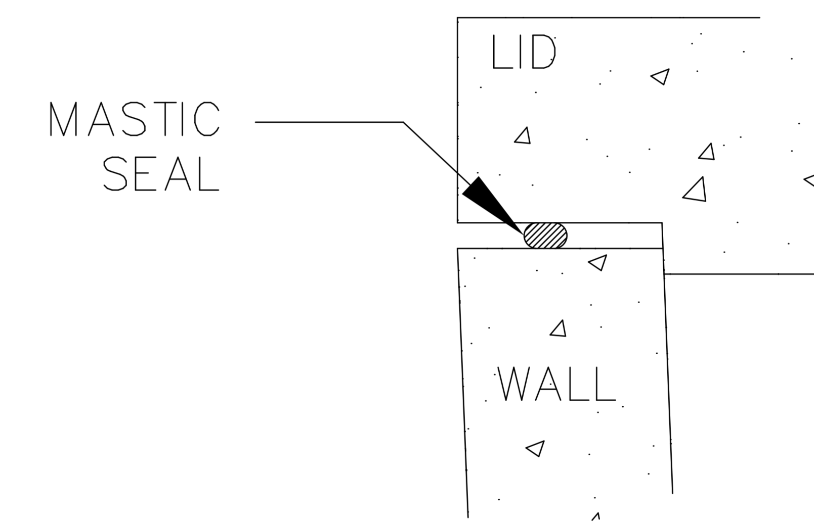
SEAL DETAIL
