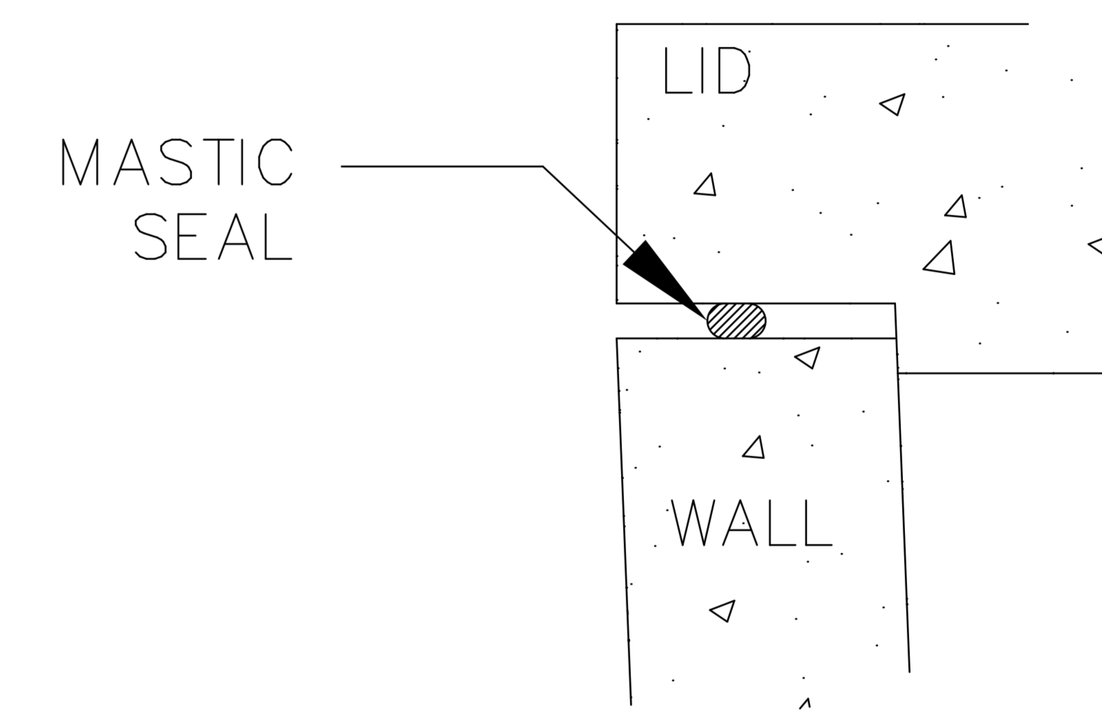
SEAL DETAIL
