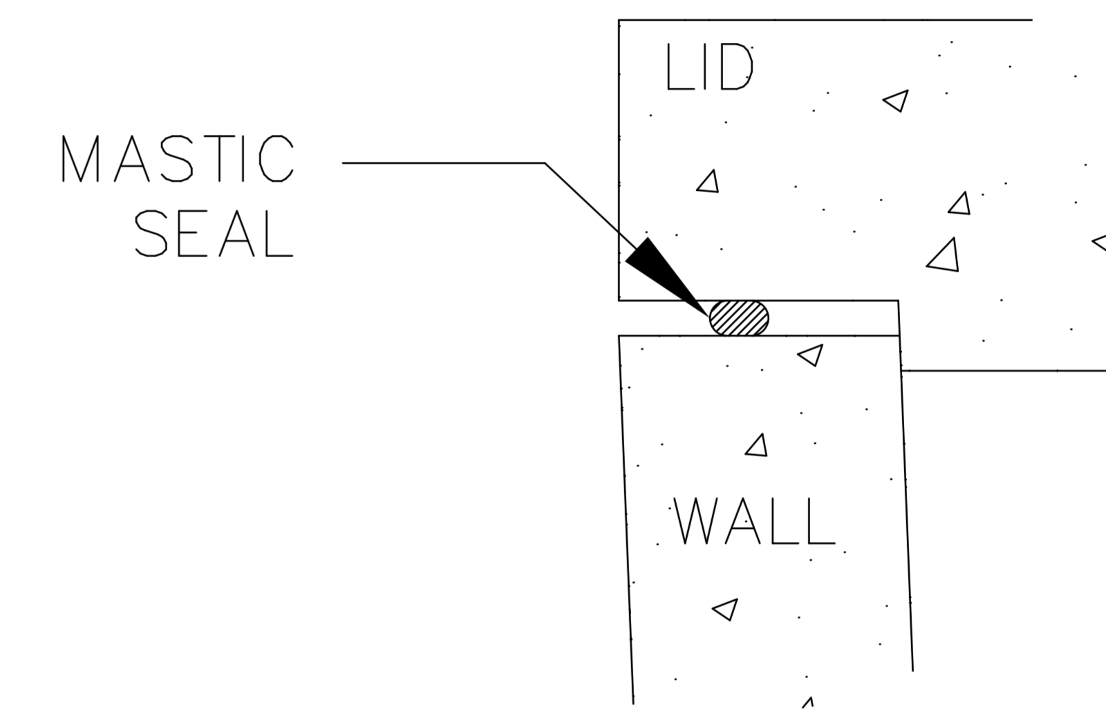
SEAL DETAIL
