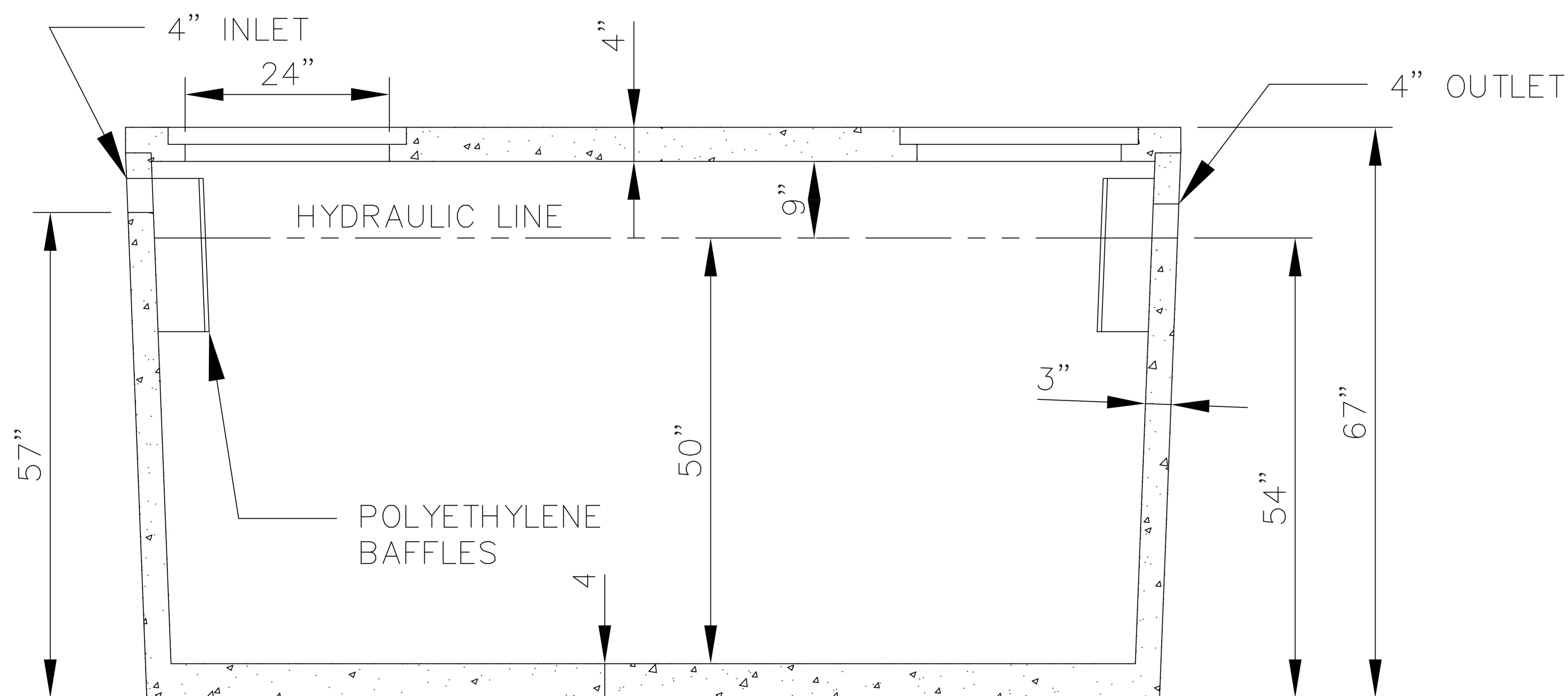
SECTION VIEW
