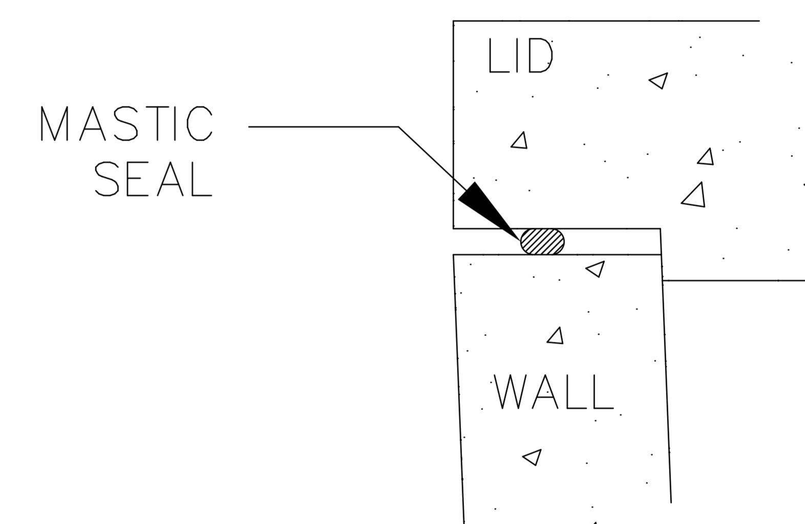
SEAL DETAIL
