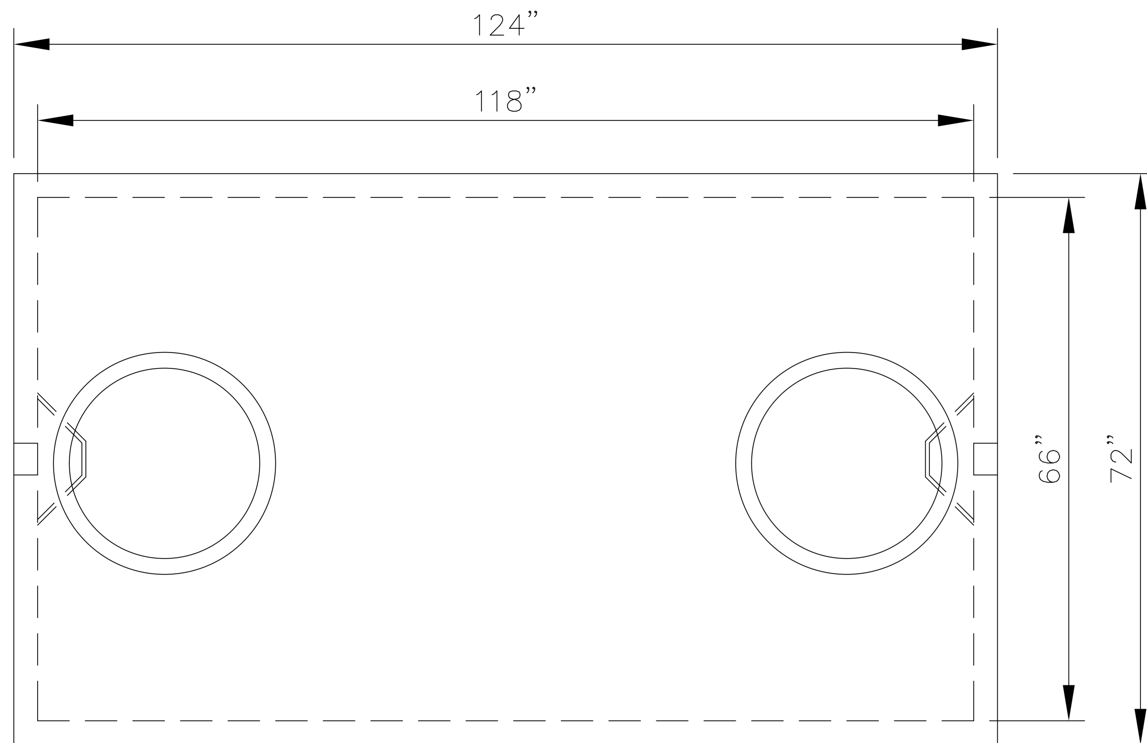
PLAN VIEW
