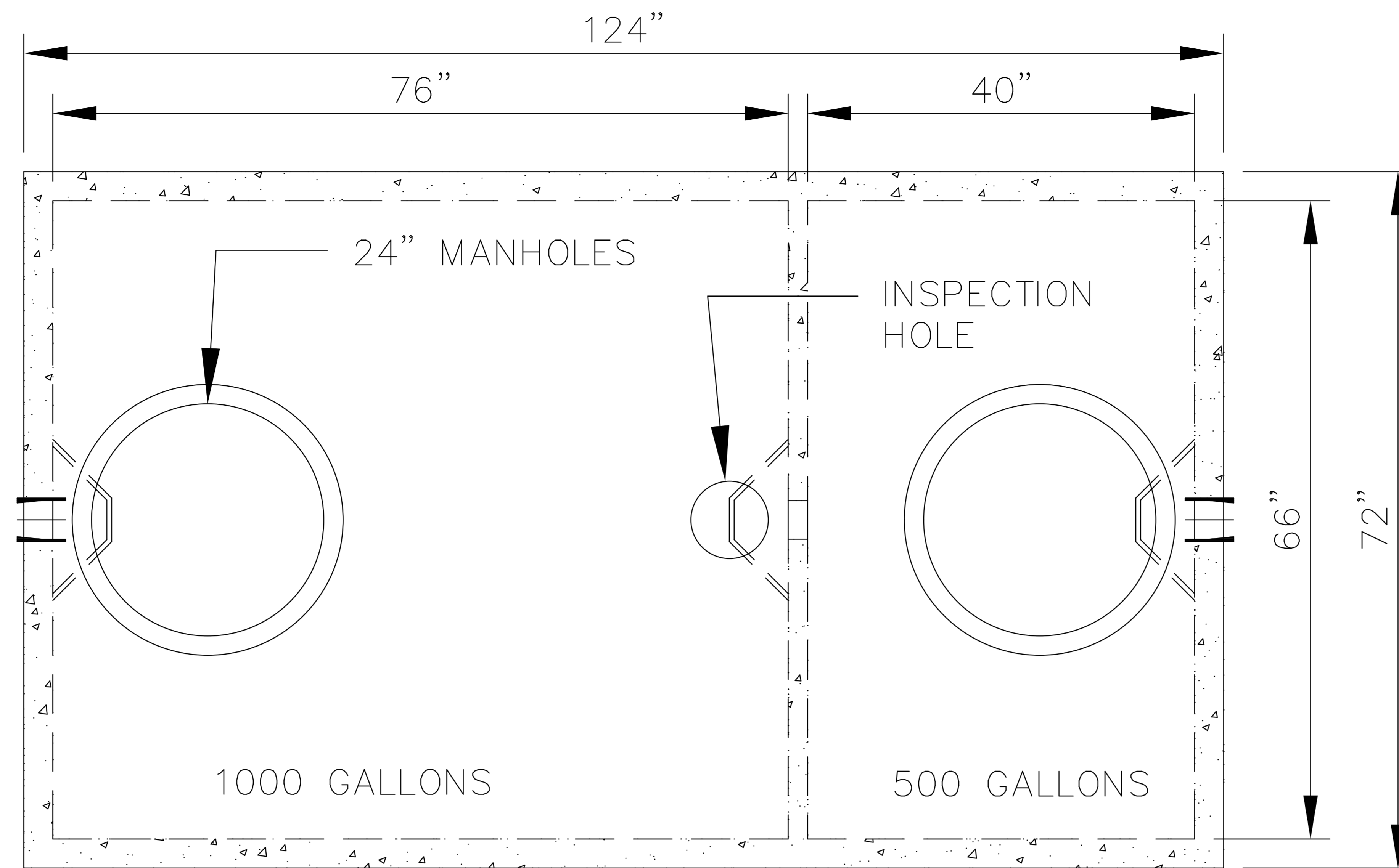
PLAN VIEW
