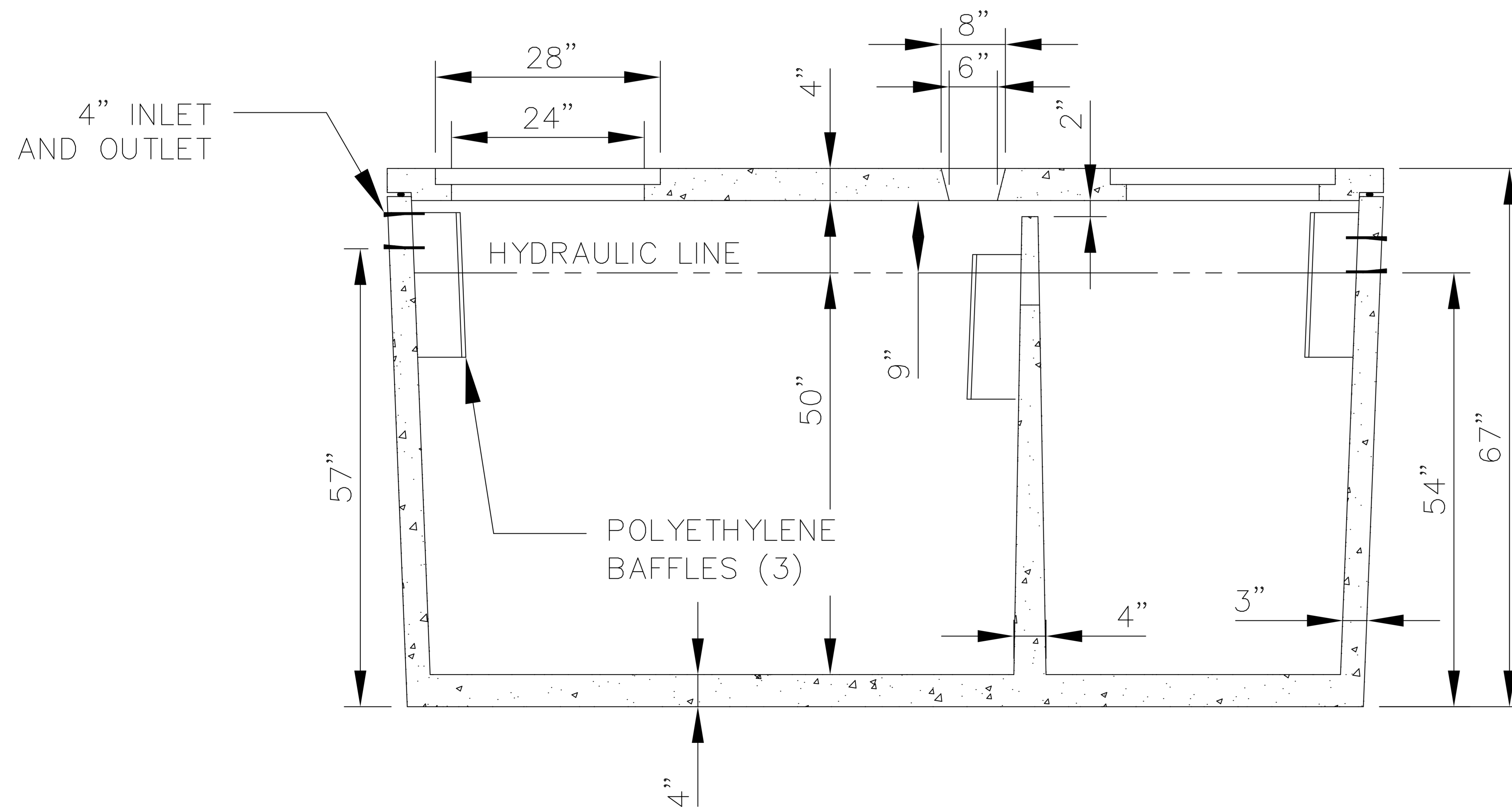
SECTION VIEW
