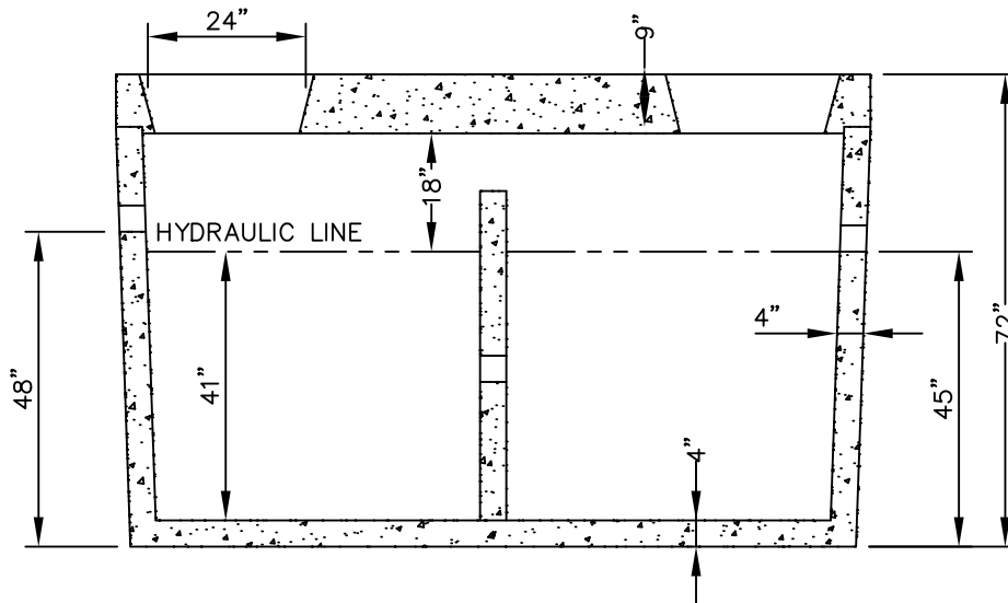
SECTION VIEW
