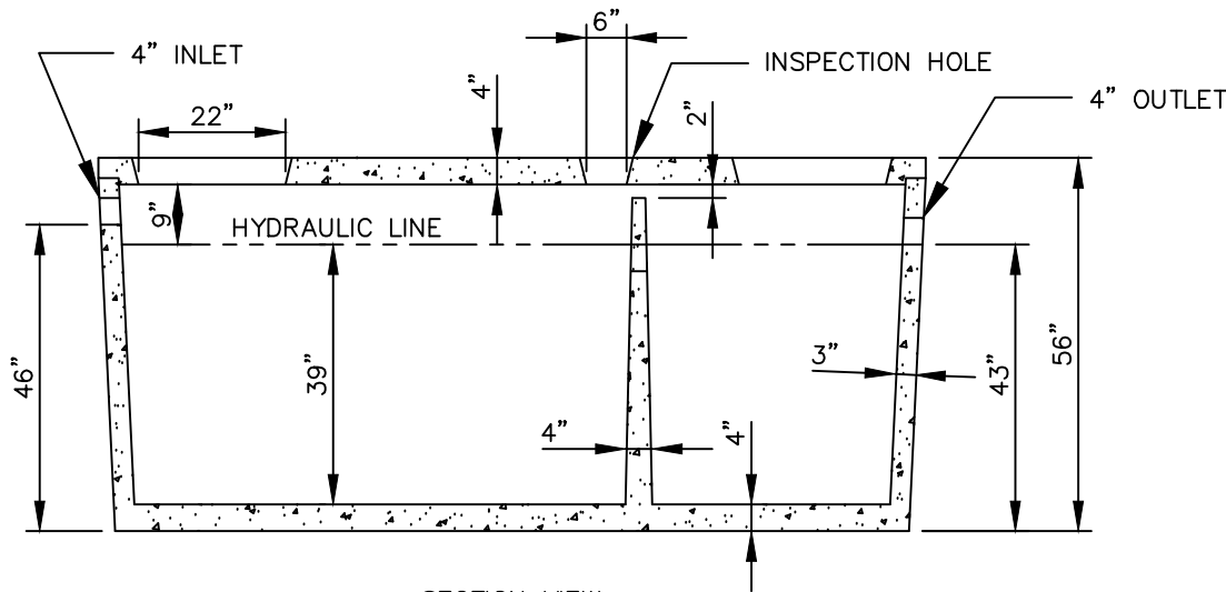
SECTION VIEW
