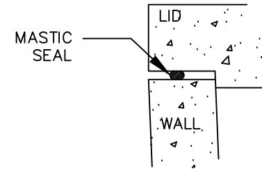
SEAL DETAIL
